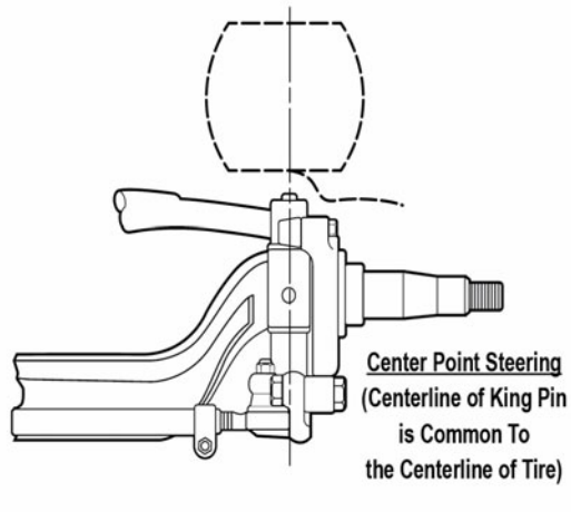
COE (FLP, FLT)
